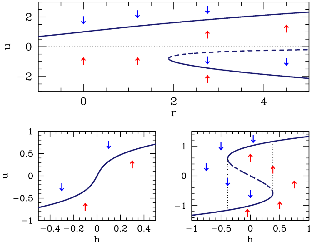
Figure 7.30: Top: extended phase space (r, u) flow diagram for \dot{u} = h + ru - u^3 , the imperfect pitchfork bifurcation, at h = 1 . This is in a sense a deformed supercritical pitchfork. The saddle-node bifurcation occurs at r_c = (3/2^{2/3})|h|^{2/3} = 1.8899 . Bottom: extended phase space (h, u) flow diagram for the imperfect pitchfork bifurcation r = -0.2 (left panel) and r = 1 (right panel). For r < 0 the behavior is completely reversible. For r > 0 , a regime of irreversibility sets in between -h_c and +h_c , where h_c = 2(r/3)^{3/2} . The system then exhibits the phenomenon of hysteresis. The dotted vertical lines show the boundaries of the hysteresis loop.
