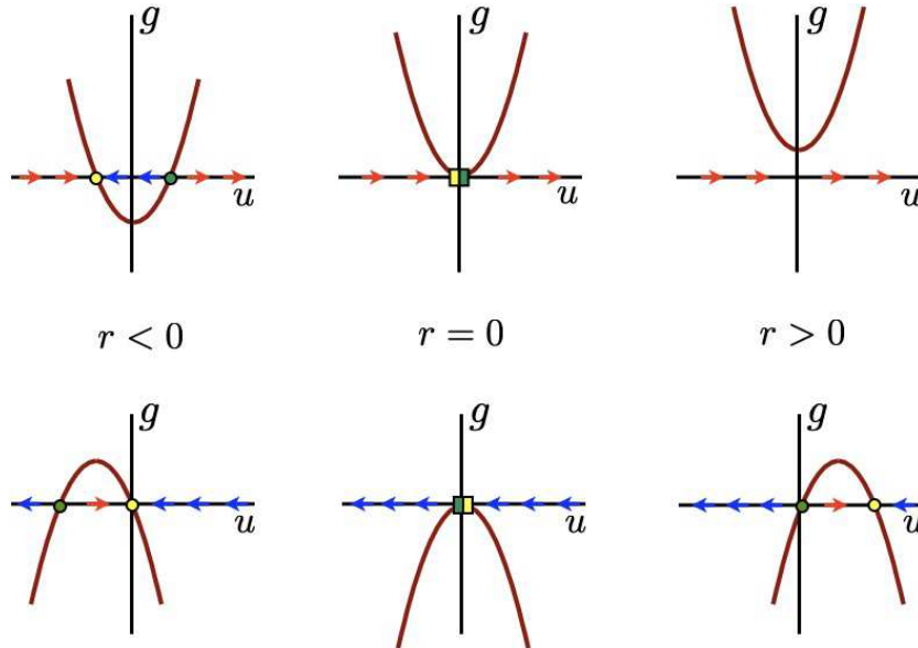
Figure 7.25: Flow diagrams for the saddle-node bifurcation \dot{u} = r + u^2 (top) and the transcritical bifurcation \dot{u} = ru - u^2 (bottom).
