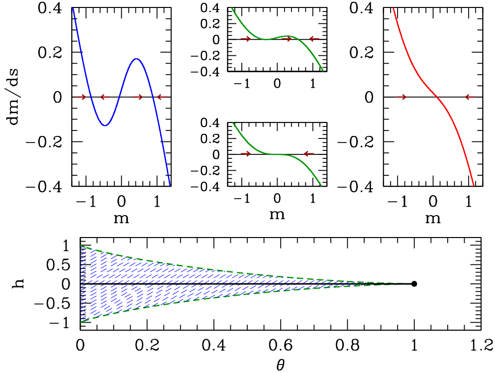
Figure 7.11: Dissipative magnetization dynamics \dot{m} = -f'(m) . Bottom panel shows h^*(\theta) from eqn. 7.79. For (\theta, h) within the blue shaded region, the free energy f(m) has a global minimum plus a local minimum and a local maximum. Otherwise f(m) has only a single global minimum. Top panels show an imperfect bifurcation in the magnetization dynamics at h = 0.0215 , for which \theta^* = 0.90 . Temperatures shown: \theta = 0.65 (blue), \theta = \theta^*(h) = 0.90 (green), and \theta = 1.2 . The rightmost stable fixed point corresponds to the global minimum of the free energy. The bottom of the middle two upper panels shows h = 0 , where both of the attractive fixed points and the repulsive fixed point coalesce into a single attractive fixed point (supercritical pitchfork bifurcation).
