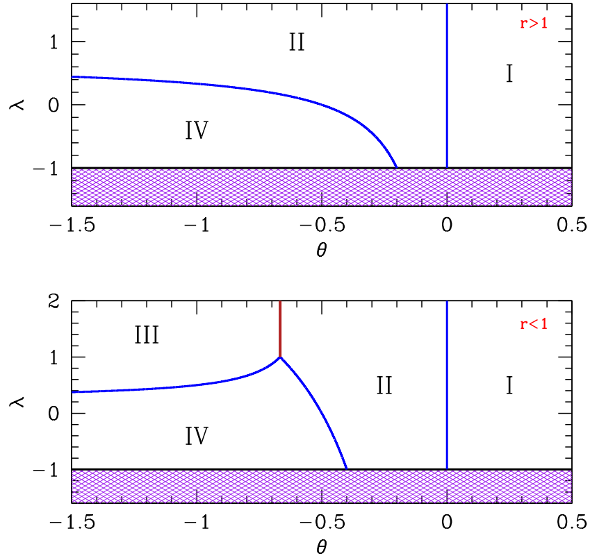
Figure 7.35: Phase diagram for \tau = 0.5 , r = 1.5 (top) and \tau = 0.5 , r = 0.25 (bottom). The hatched purple region is unphysical, with a free energy unbounded from below. The blue lines denote second order transitions. The thick red line separating phases II and III is a first order line.
