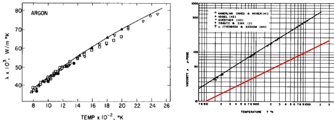
Figure 8.5: Left: thermal conductivity ( \lambda in figure) of Ar between T = 800 \text{ K} and T = 2600 \text{ K} . The best fit to a single power law \lambda = aT^b results in b = 0.651 . Source: G. S. Springer and E. W. Wingeier, J. Chem Phys. 59 , 1747 (1972). Right: log-log plot of shear viscosity ( \mu in figure) of He between T \approx 15 \text{ K} and T \approx 1000 \text{ K} . The red line has slope \frac{1}{2} . The slope of the data is approximately 0.633. Source: J. Kestin and W. Leidenfrost, Physica 25 , 537 (1959).
