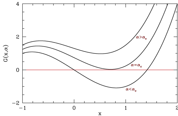
Figure 7.24: Evolution of G(x, \alpha) as a function of the control parameter \alpha .
