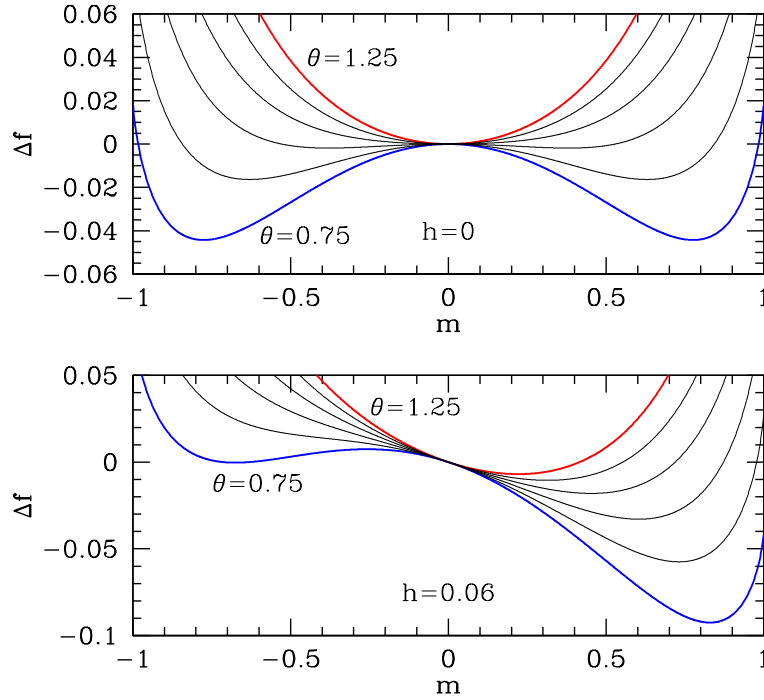
Figure 7.19: Variational field free energy \Delta f = f(m, \theta, h) + \theta \log 2 versus magnetization m at six equally spaced temperatures interpolating between ‘high’ ( \theta = 1.25 , red) and ‘low’ ( \theta = 0.75 , blue) values. Top panel: h = 0 . Bottom panel: h = 0.06 .
