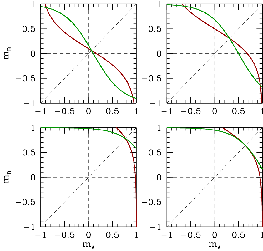
Figure 7.32: Graphical solution to the mean field equations for the Ising antiferromagnet in an external field, here for \theta = 0.6 . Clockwise from upper left: (a) h = 0.1 , (b) h = 0.5 , (c) h = 1.1 , (d) h = 1.4 .
