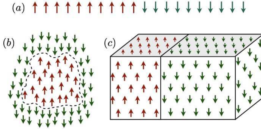
Figure 7.21: Domain walls in the (a) d = 1 , (b) d = 2 , and (c) d = 3 Ising model.
