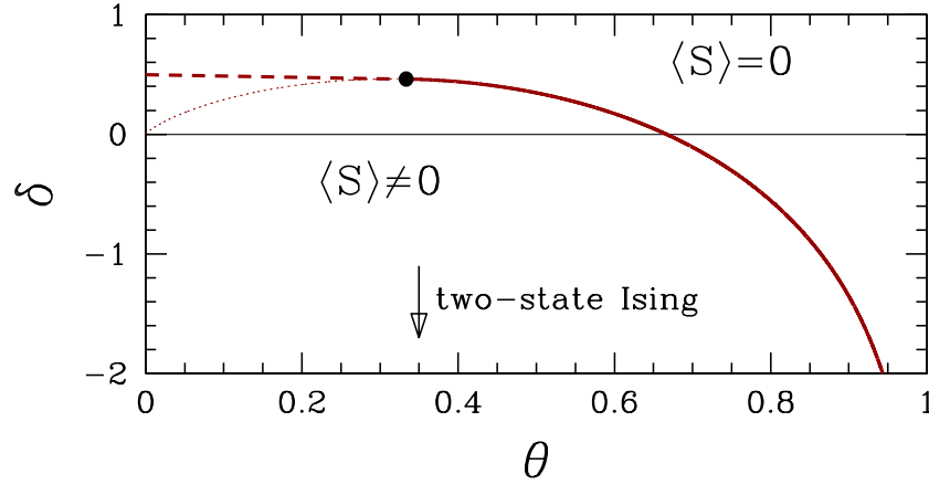
Figure 7.31: Mean field phase diagram for the Blume-Capel model. The black dot signifies a tricritical point, where the coefficients of m^2 and m^4 in the Landau free energy expansion both vanish. The dashed curve denotes a first order transition, and the solid curve a second order transition. The thin dotted line is the continuation of the \delta^*(\theta) relation to zero temperature.
