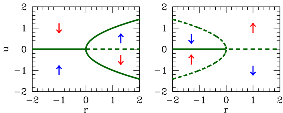
Figure 7.28: Extended phase space (r, u) flow diagrams for the pitchfork bifurcation. Left: supercritical pitchfork \dot{u} = ru - u^3 . Right: subcritical pitchfork \dot{u} = ru + u^3 .
