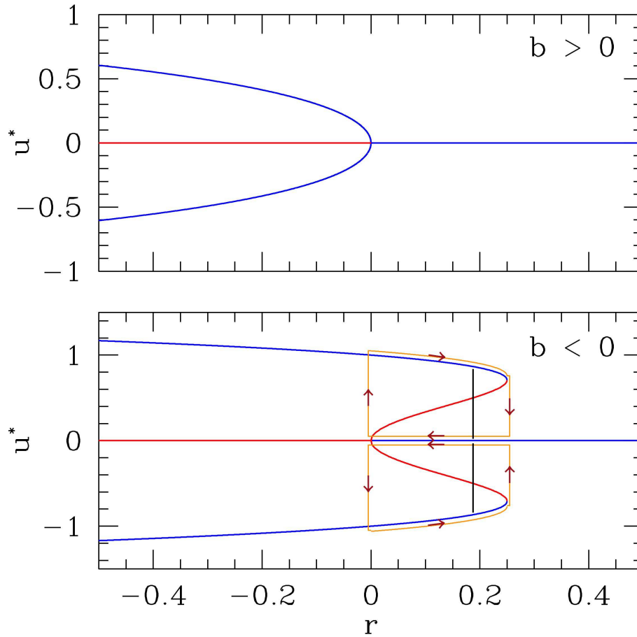
Figure 7.18: Fixed points branches \varphi'(u^*) = 0 for the sextic potential \varphi(u) = \frac{1}{2}ru^2 + \frac{\sigma}{4}u^4 + \frac{1}{6}u^6 with \sigma = \text{sgn}(b) (top for \sigma = +1 , bottom for \sigma = -1 ). Blue curves indicate stable branches and red unstable branches under the dynamics \dot{u} = -\varphi'(u) . For b > 0 there is a supercritical pitchfork bifurcation at (0,0) and no hysteresis. For b < 0 there is a subcritical pitchfork bifurcation at (0,0) and two saddle-node bifurcations at (\frac{1}{4}, \pm\frac{1}{\sqrt{2}}) . Solid curves show stable fixed points and dashed curves show unstable fixed points. The thick solid black segment indicates the order parameter discontinuity in u at the thermodynamic first order phase transition. Note the overall u \rightarrow -u symmetry. Within the region r \in [0, \frac{1}{4}] the dynamics are irreversible and the system exhibits the phenomenon of hysteresis. There is a first order phase transition at r = \frac{3}{16} , indicated by the thick black line segment which shows the discontinuous jump of the order parameter u at the transition.
