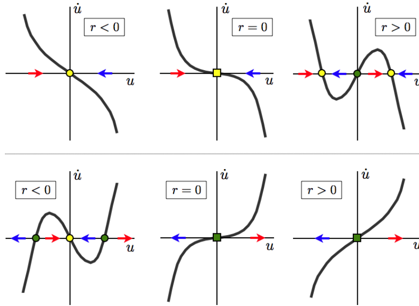
Figure 7.27: Top: supercritical pitchfork bifurcation \dot{u} = ru - u^3 . Bottom: subcritical pitchfork bifurcation \dot{u} = ru + u^3 .
