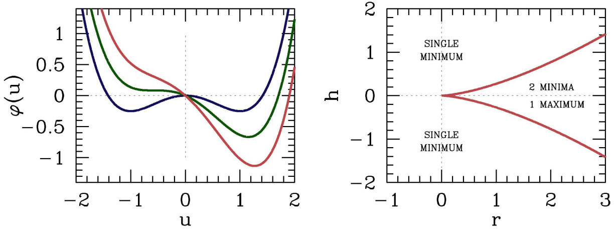
Figure 7.29: Left: scaled free energy \phi(u) = -\frac{1}{2}ru^2 + \frac{1}{4}u^4 - hu , with h = 0 (blue), h = h_c (green), and h = 2h_c (red), where h_c = \frac{2}{3\sqrt{3}}r^{3/2} . Right: phase diagram for the imperfect bifurcation \dot{u} = -\phi'(u) = h + ru - u^3 in the (r, h) plane.
