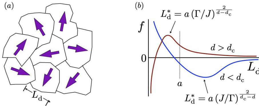
Figure 7.23: (a) Imry-Ma domains for an O(2) model. The arrows point in the direction of the local order parameter field \langle \hat{n}(\mathbf{r}) \rangle . (b) Free energy density as a function of domain size L_d . Keep in mind that the minimum possible value for L_d is the lattice spacing a .
