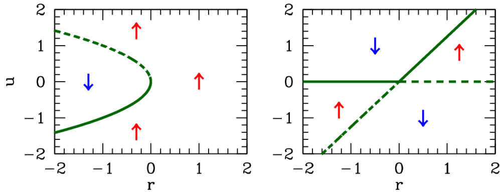
Figure 7.26: Extended phase space (r, u) flow diagrams for the saddle-node bifurcation \dot{u} = r + u^2 (left) and the transcritical bifurcation \dot{u} = ru - u^2 (right).
