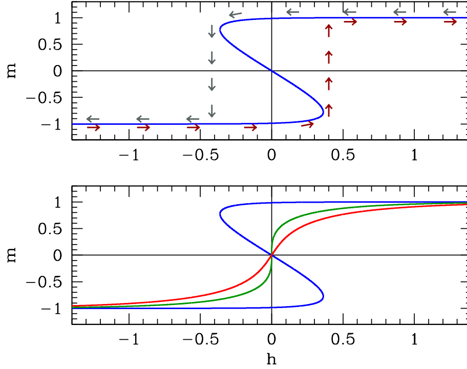
Figure 7.12: Top panel: hysteresis as a function of ramping the dimensionless magnetic field h at \theta = 0.40 . Dark red arrows below the curve track the evolution of m upon a slow increase of h . Dark grey arrows above the curve track a slow decrease of h . Bottom panel: solution set for m(\theta, h) as a function of h at temperatures \theta = 0.40 (blue), \theta = \theta_c = 1.0 (dark green), and t = 1.25 (red).
