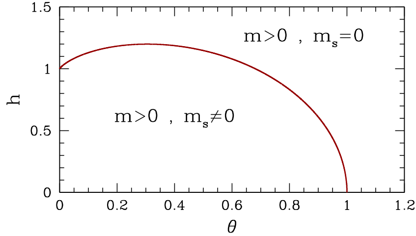
Figure 7.33: Mean field phase diagram for the Ising antiferromagnet in an external field. The phase diagram is symmetric under reflection in the h = 0 axis.
